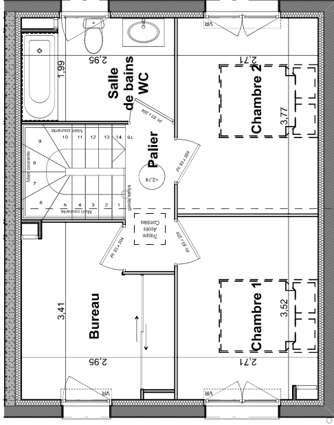
PLAN R+1 Ech: 1/100
